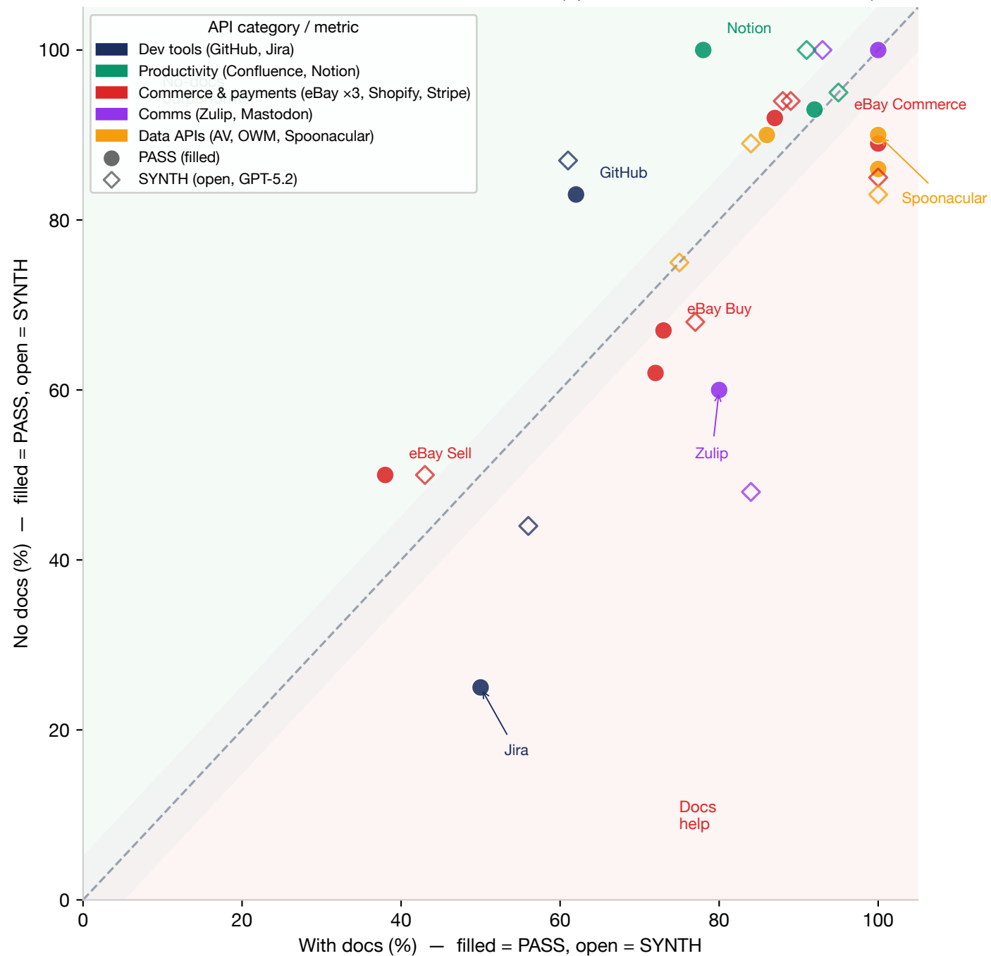
Effect of documentation on PASS and SYNTH (open markers = SYNTH, GPT-5.2)
