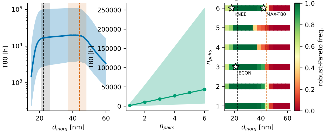
(a) 95% CI band; threshold (b) Pair law: linear in all 500 draws (c) Robust design map 22.5 [21-26] / 44 [38-48] (min R^2=0.9998 ); abs. scale \leftarrow M_{cne}^{org}=100 nm slice)
