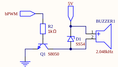
Buzzer
