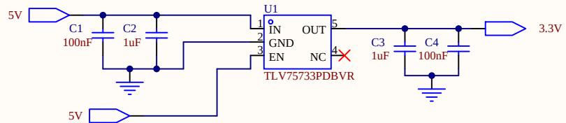
3.3V LDO
