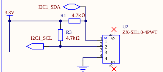
I2 SH1.0-4PWT
