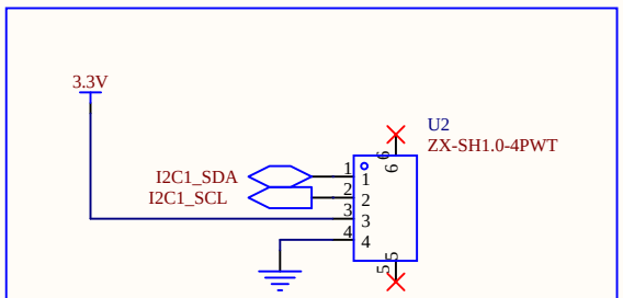
Interface SH1.0-4PWT
