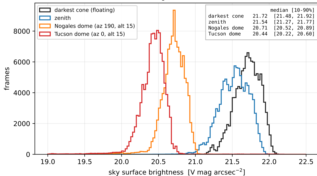
clear-night distributions
