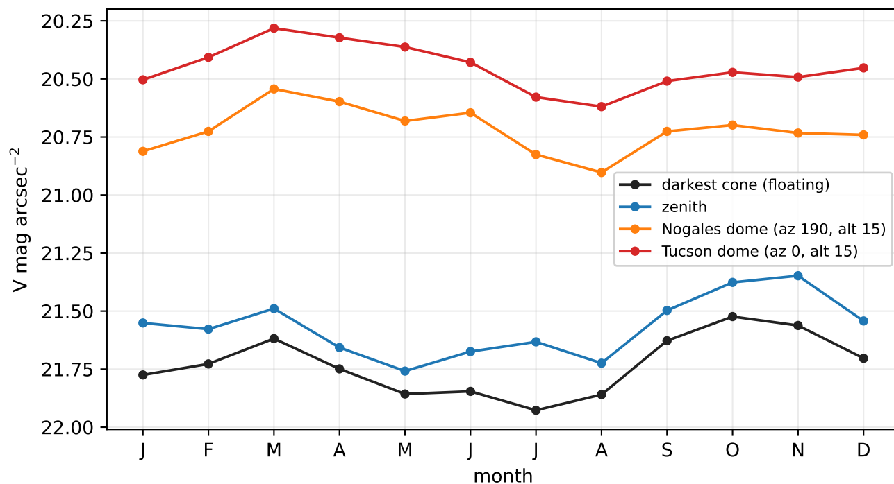
seasonal medians
