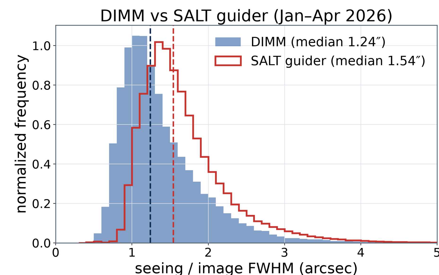
Normalized distributions of DIMM seeing ( n = 33,087 ) and SALT guider image FWHM ( n = 352,555 ) over the Jan-Apr 2026 overlap period. SALT guider data includes both RSS and HRS.
