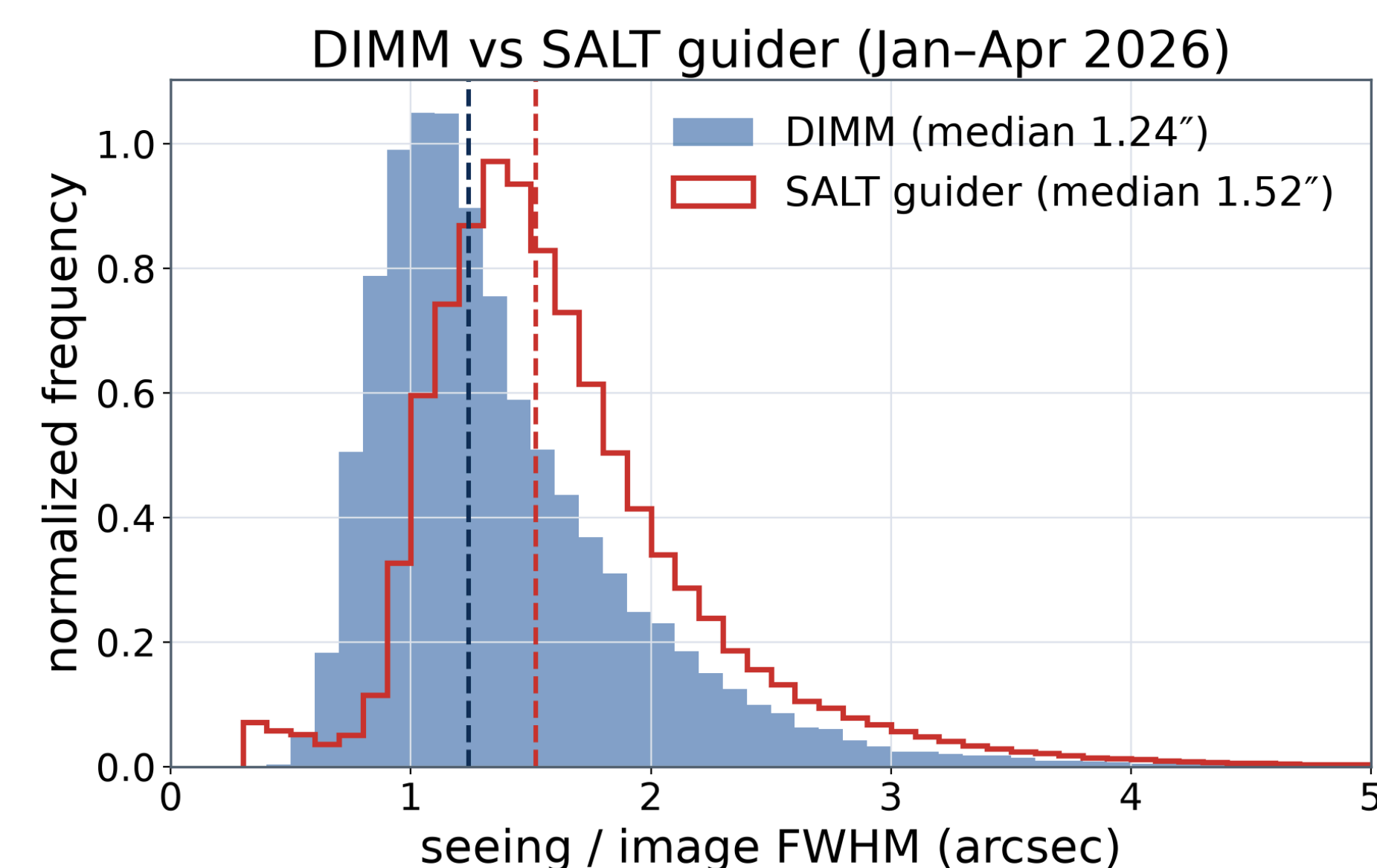
Normalized distributions of DIMM seeing ( n = 33,091 ) and SALT guider image FWHM ( n = 382,526 ), both in arcsec, over the Jan-Apr 2026 overlap. SALT guider data includes both RSS and HRS.
