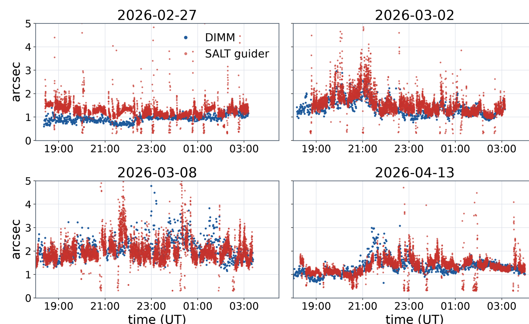
Four representative nights: DIMM seeing and SALT guider FWHM vs time.
