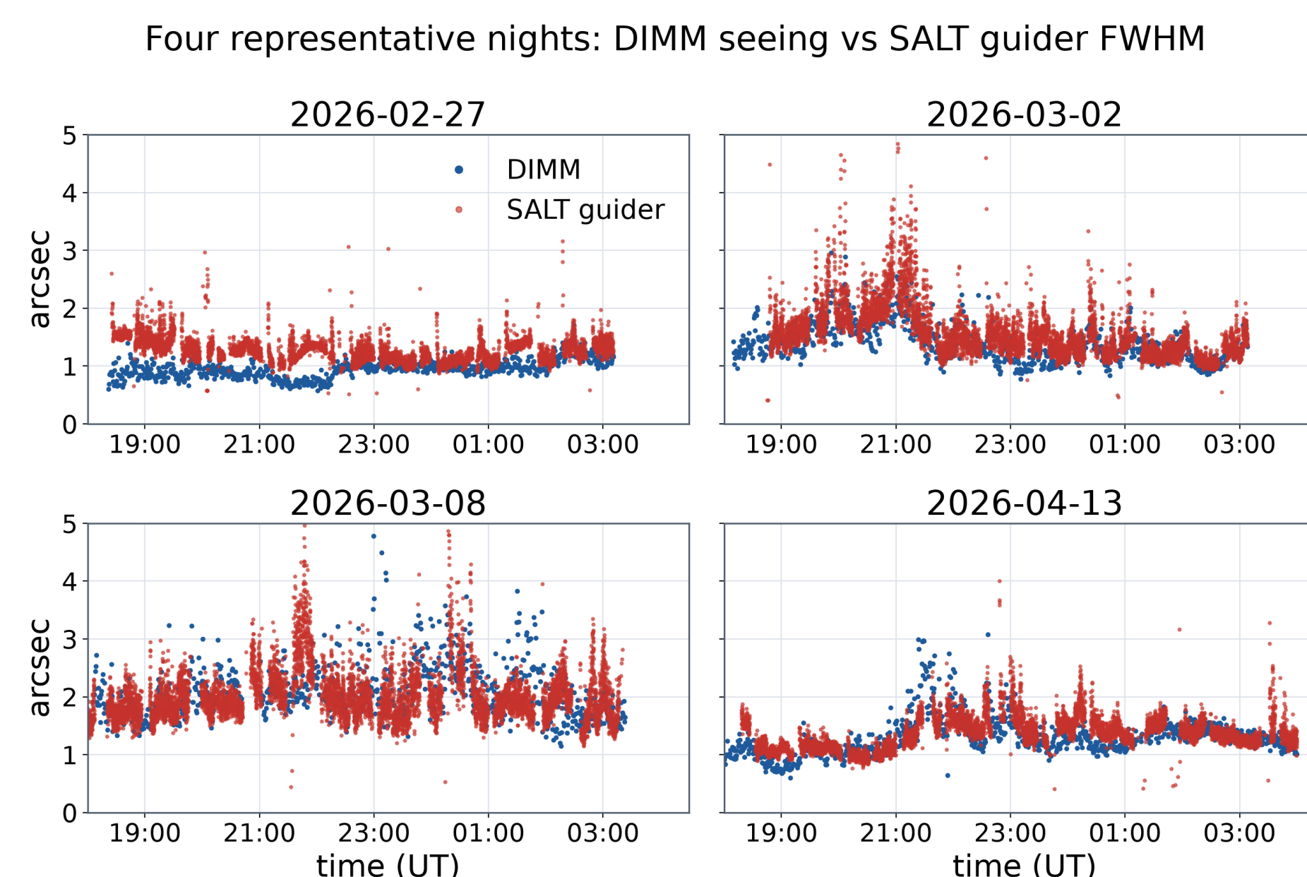
Time-series comparison of DIMM seeing and SALT guider FWHM for four representative, clear nights.
