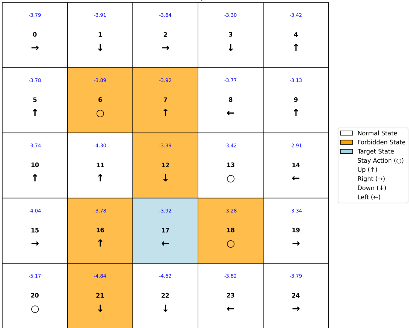
Grid World Environment with Policy and State Value
