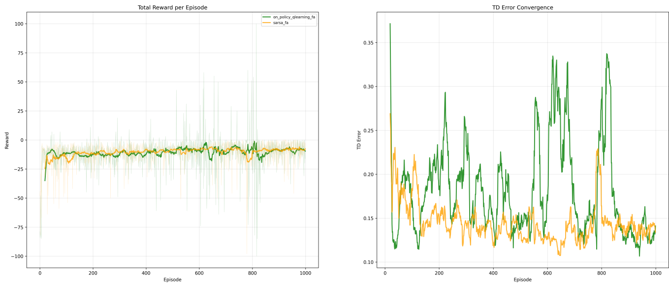
Multi-Algorithm Training Comparison
