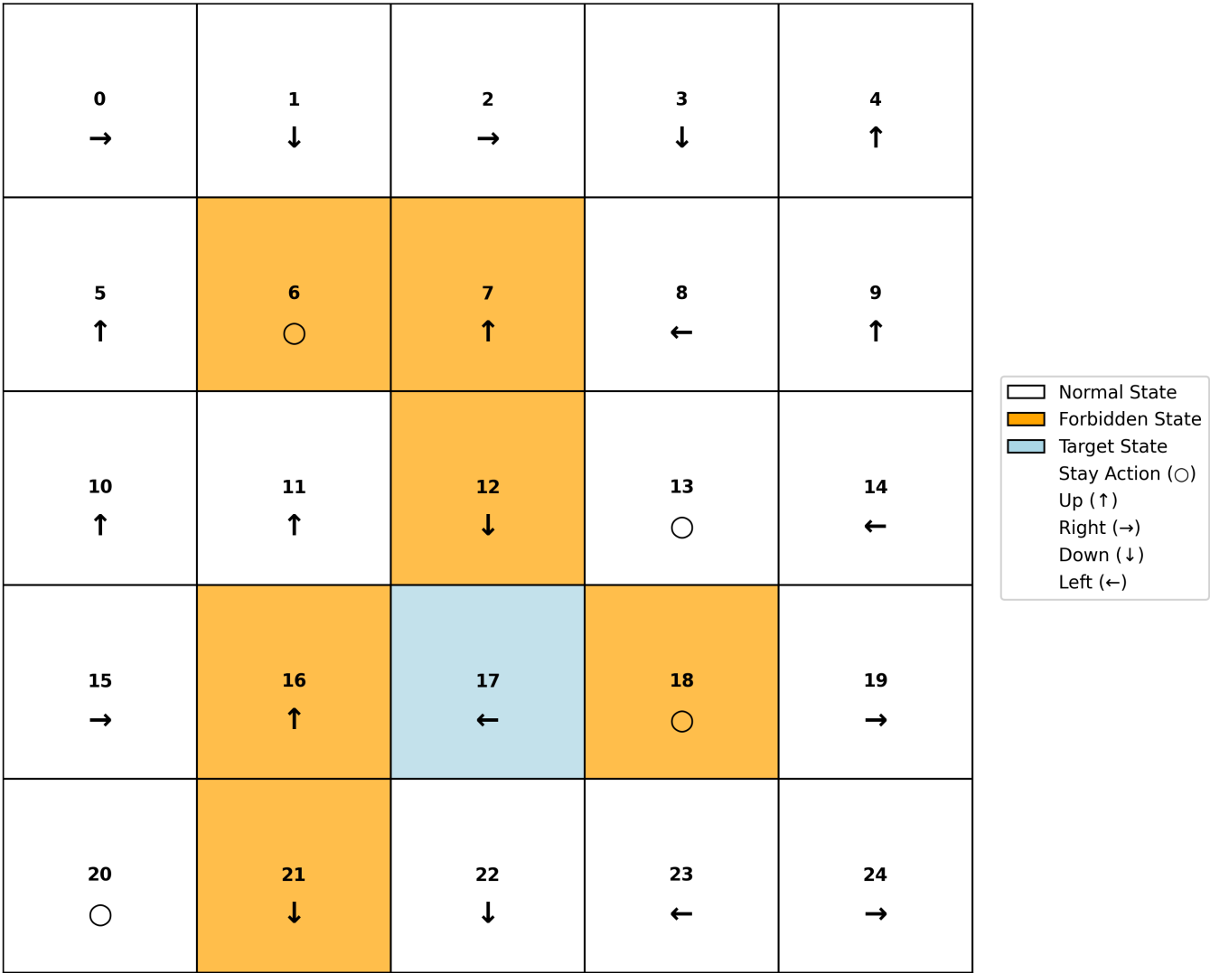
Grid World Environment with Policy
