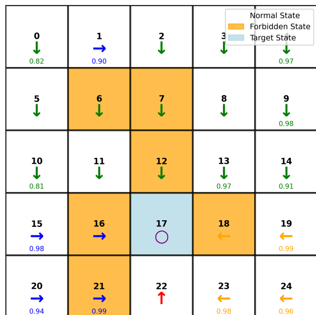
REINFORCE Policy
