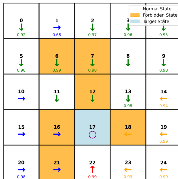
Actor-Critic Policy
