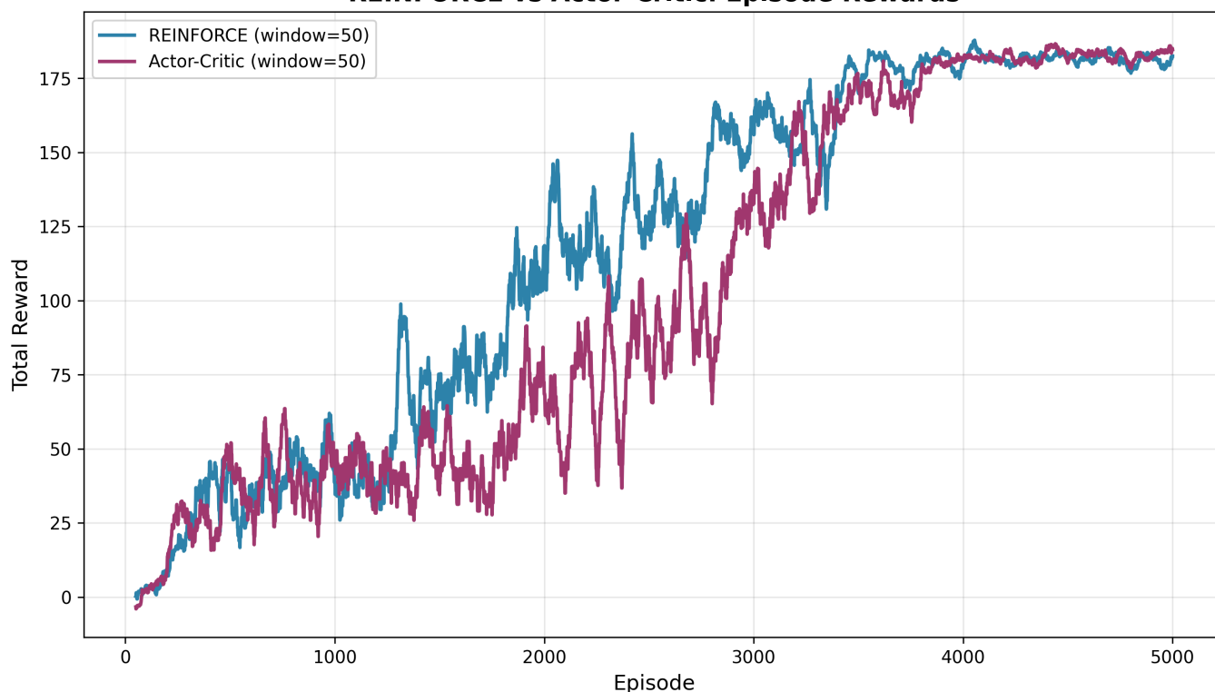
REINFORCE vs Actor-Critic: Episode Rewards
