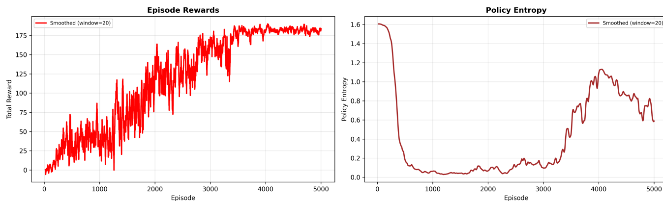
Actor-Critic Training Curves
