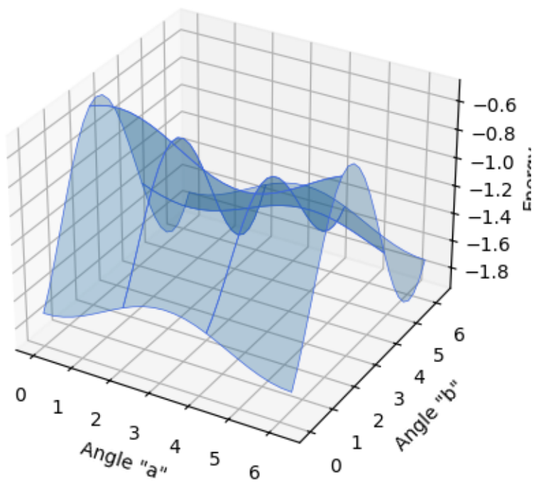
Original Hamiltonian
