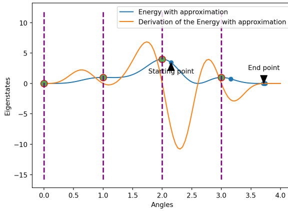
Figure 6: Energy graph Optimization with the Approximation method
