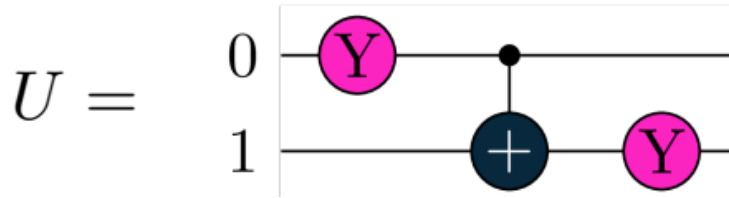
Figure 1: Circuit
