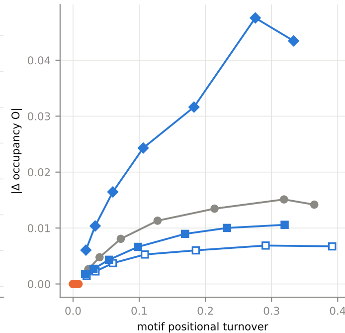
B occupancy vs motif turnover
