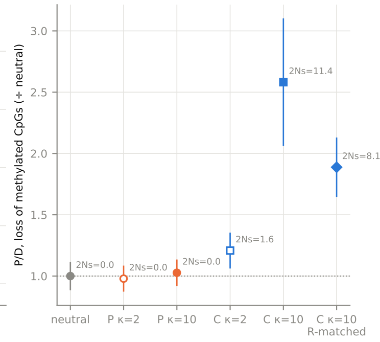
D polymorphism / divergence
