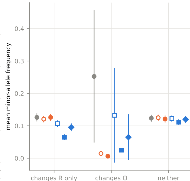
C allele frequency by effect class
