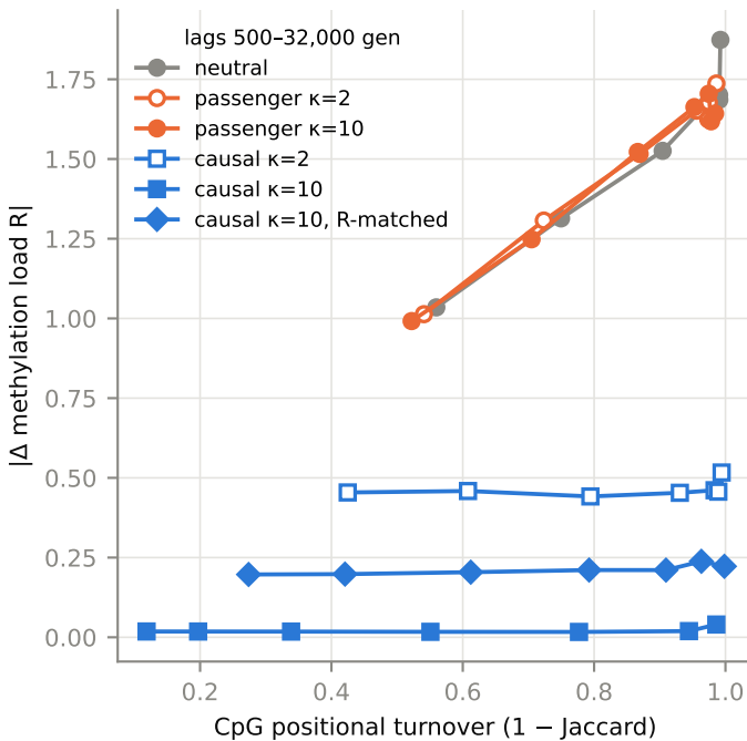
A methylation load vs CpG turnover
