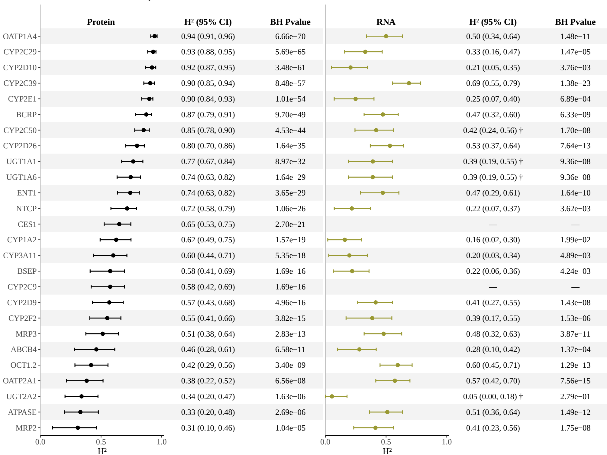
A Broad-sense heritability
