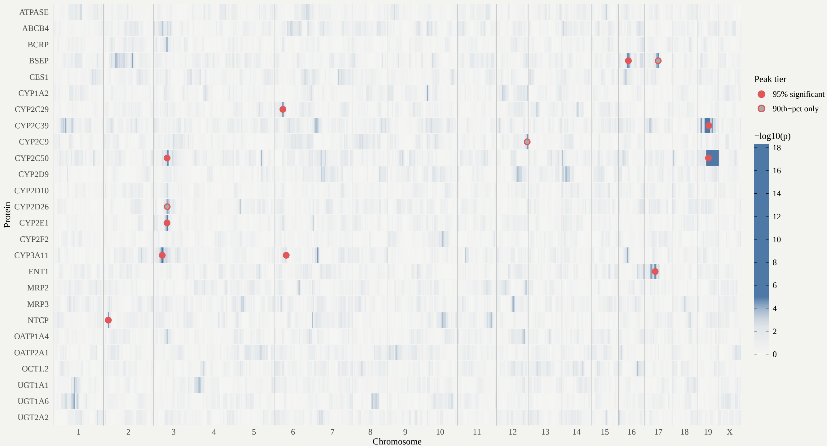
Genome-wide pQTL scan summary Tile color is -\log_{10}(p) on a continuous white-to-blue scale
