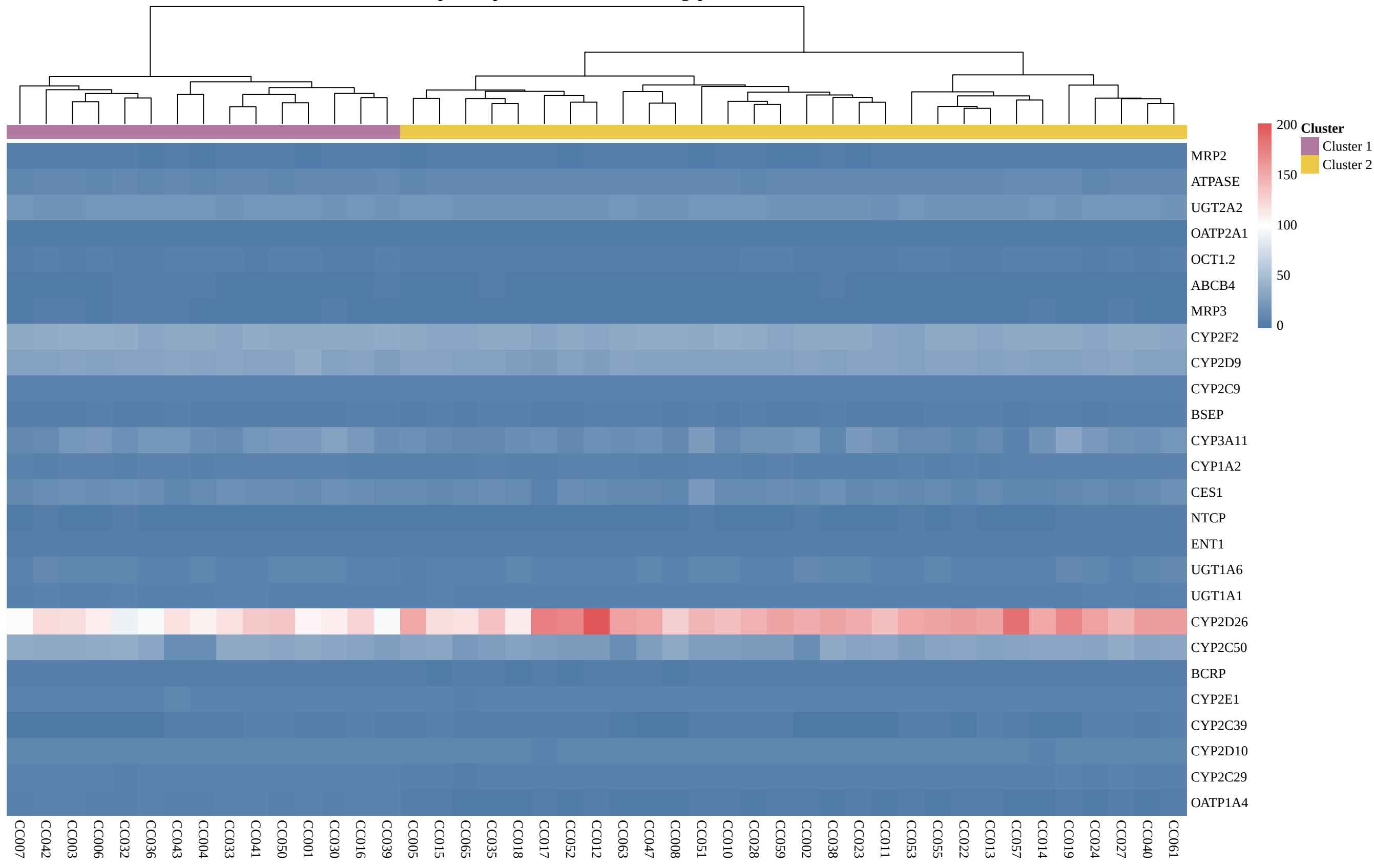
DMET protein profiles across CC strains; gap-statistic k = 2
