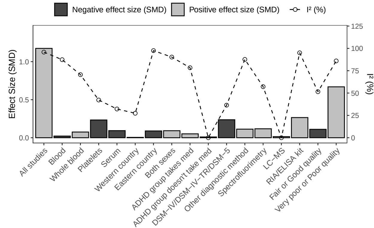
F – 5-hydroxy-indoleacetic acid
