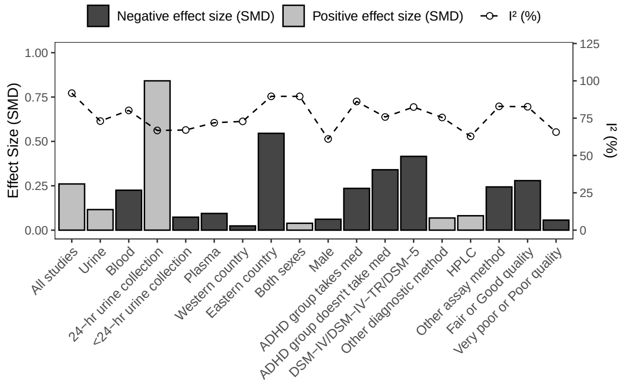
E – Homovanillic acid
