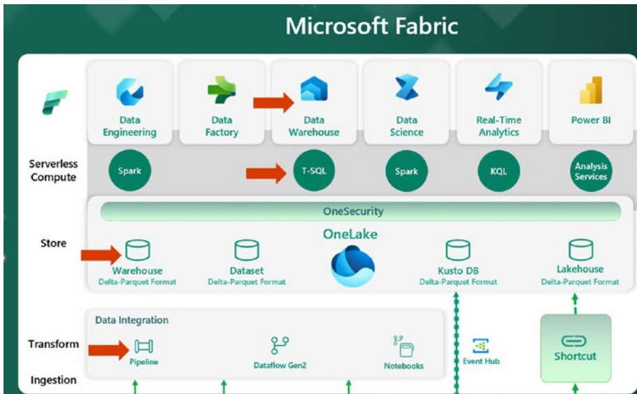
Figure 5-33. Recap of data architecture
