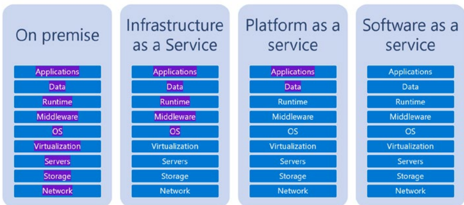
Figure 1-1. On-premises, IaaS, PaaS, and SaaS differences
