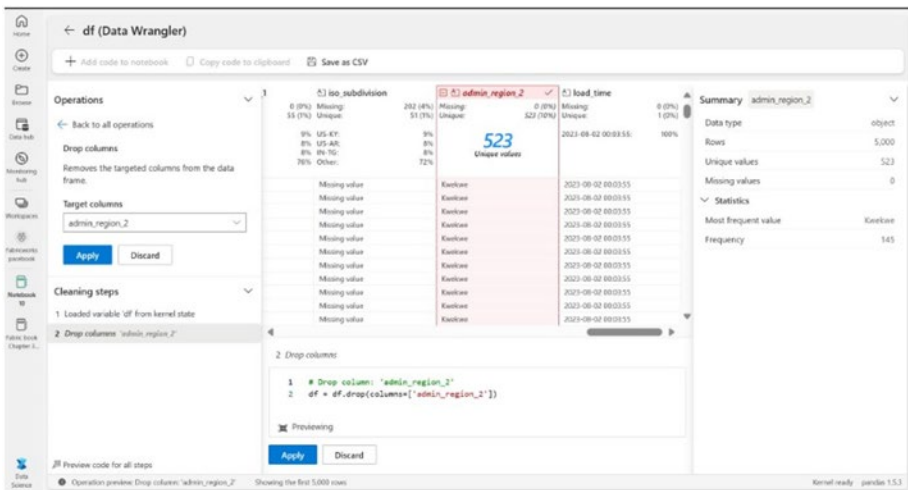
Figure 4-9. Drop column operation using Data Wrangler
