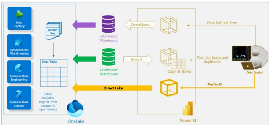
Figure 9-36. Fabric Direct Lake concept from Microsoft documentation
