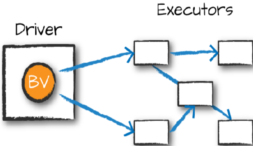
Figure 14-1. Broadcast variables
