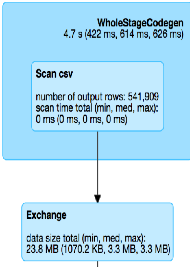
Figure 18-4. Stage one
