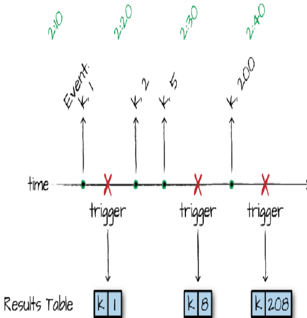
Figure 22-3. Sliding Windows
