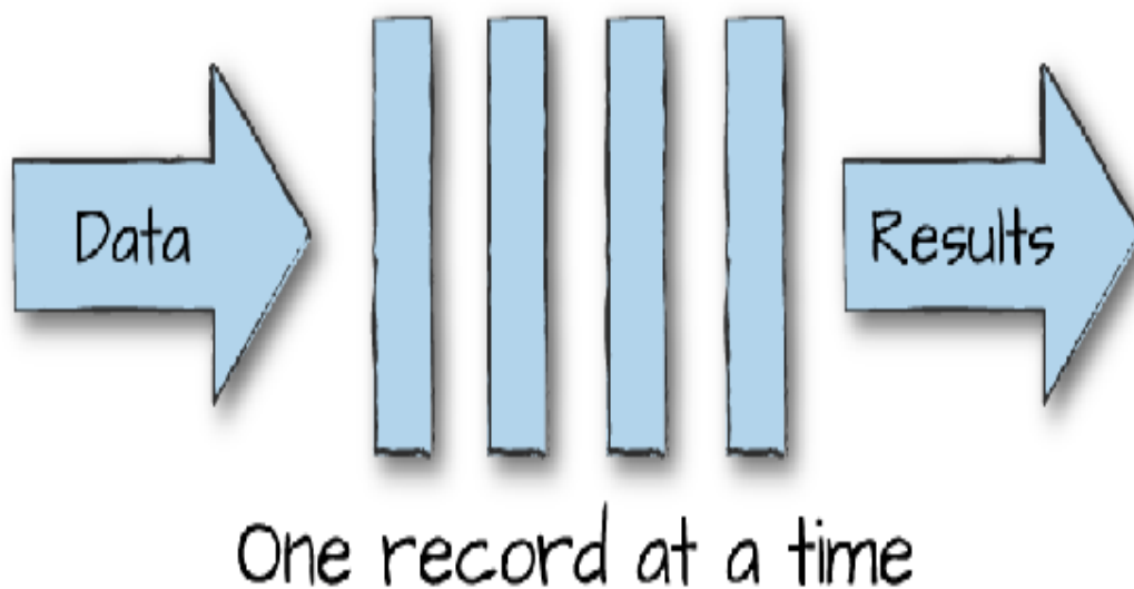
Figure 20-1. Continuous processing
