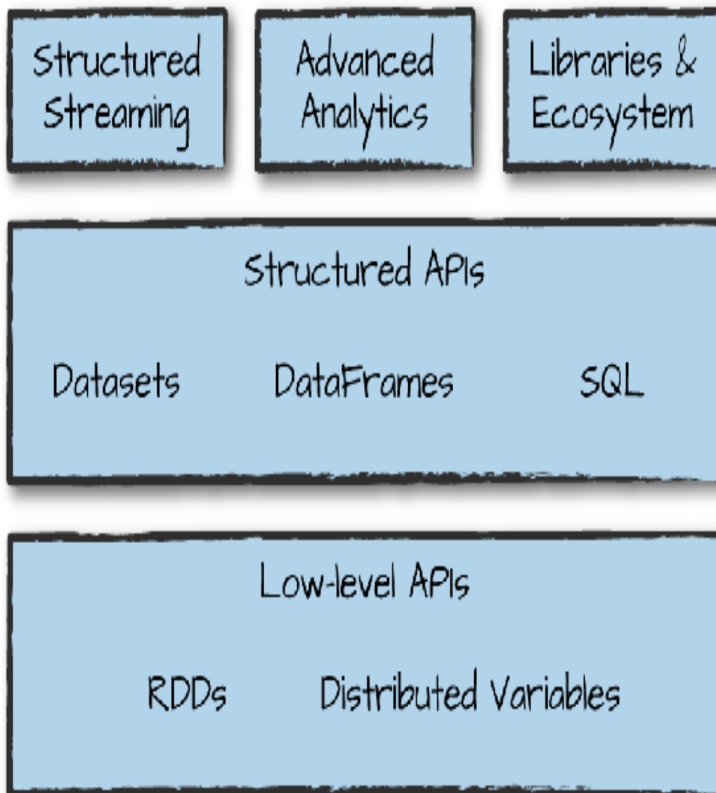
Figure 1-1. Spark's toolkit
