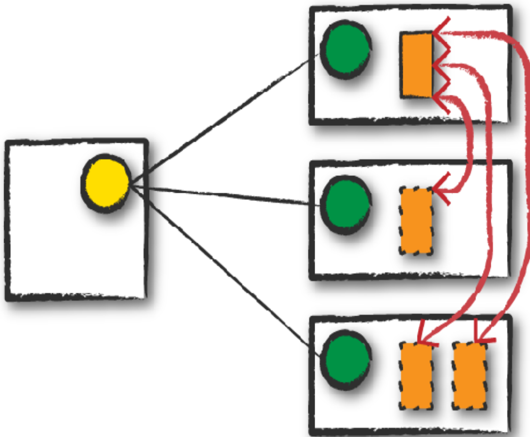
Figure 15-6. Application execution
