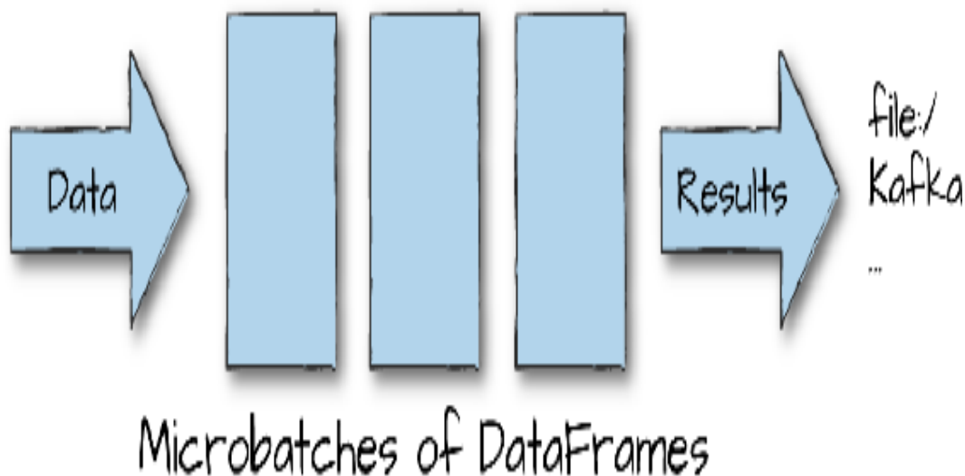
Figure 20-2. Micro-batch
