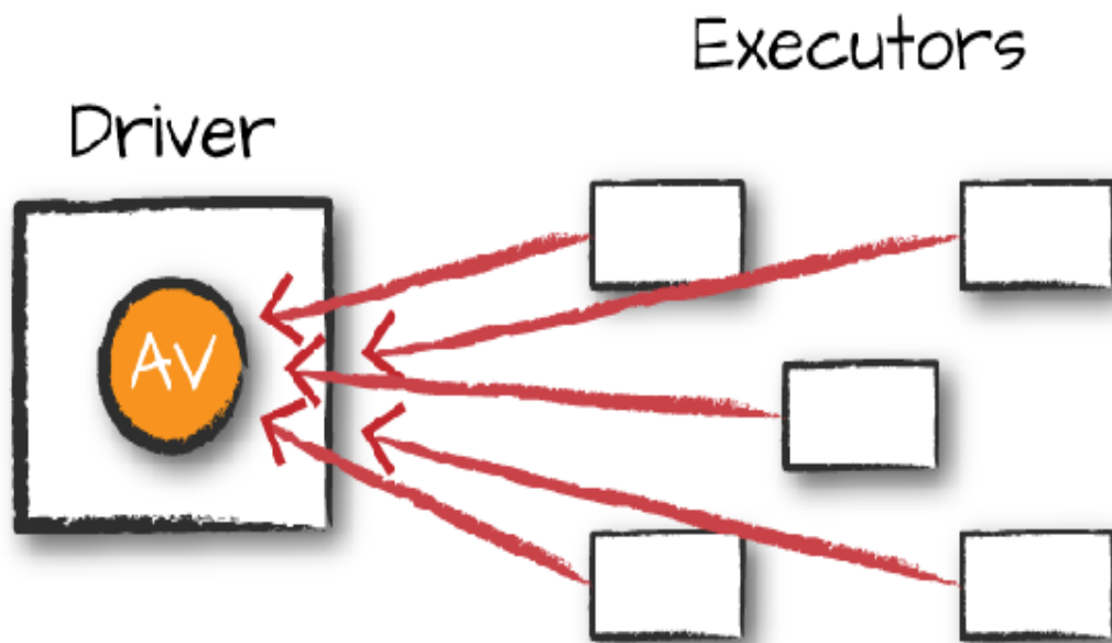
Figure 14-2. Accumulator variable
