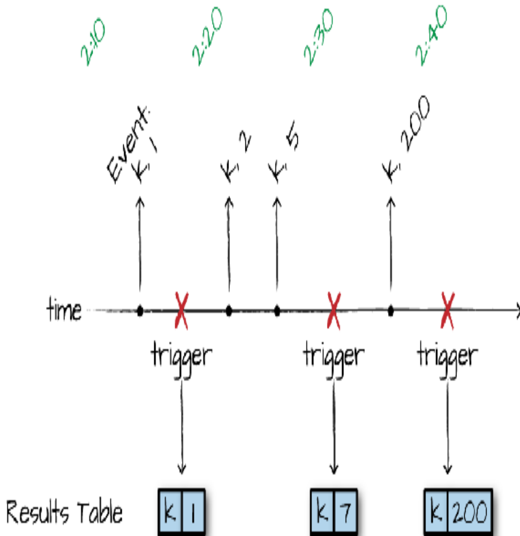
Figure 22-2. Tumbling Windows
