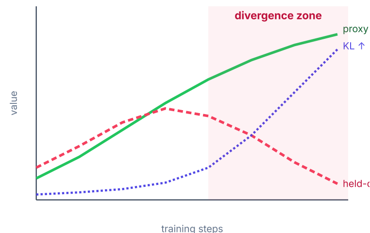
Training curve — reward hacking signature
