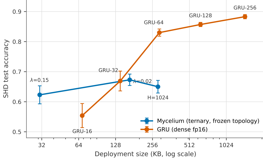
Figure 1: The memory frontier on SHD: accuracy vs. deployment size (log scale), mean \pm sd over three seeds per point. GRU points use each size’s best measured condition ( T=32 for GRU-16/32, T=64 +augmentation for GRU-64/128/256) — the baseline at its best, conservative against Mycelium. The families cross near \sim 140 KB.
