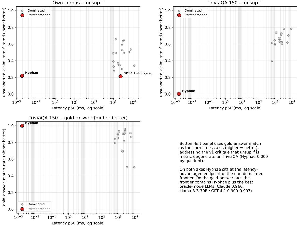
Figure 1: Latency-quality Pareto frontier on two metrics. Each point is one system configuration; latency on the horizontal axis is p_{50} in milliseconds, log scale. Top row uses unsup_f (lower better); bottom-left uses gold-answer match (higher better). Red points are non-dominated on each panel. The gold-answer panel addresses the v1 critique that unsup_f is metric-degenerate on TriviaQA for HYPHAE; the gold-answer panel surfaces the correctness comparison directly.
