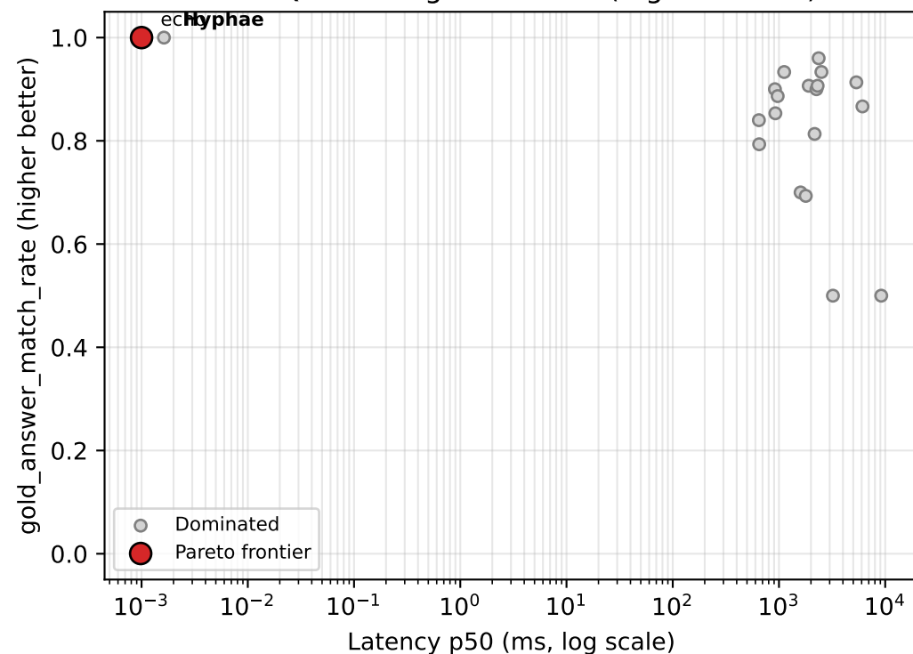
TriviaQA-150 -- gold-answer (higher better)
