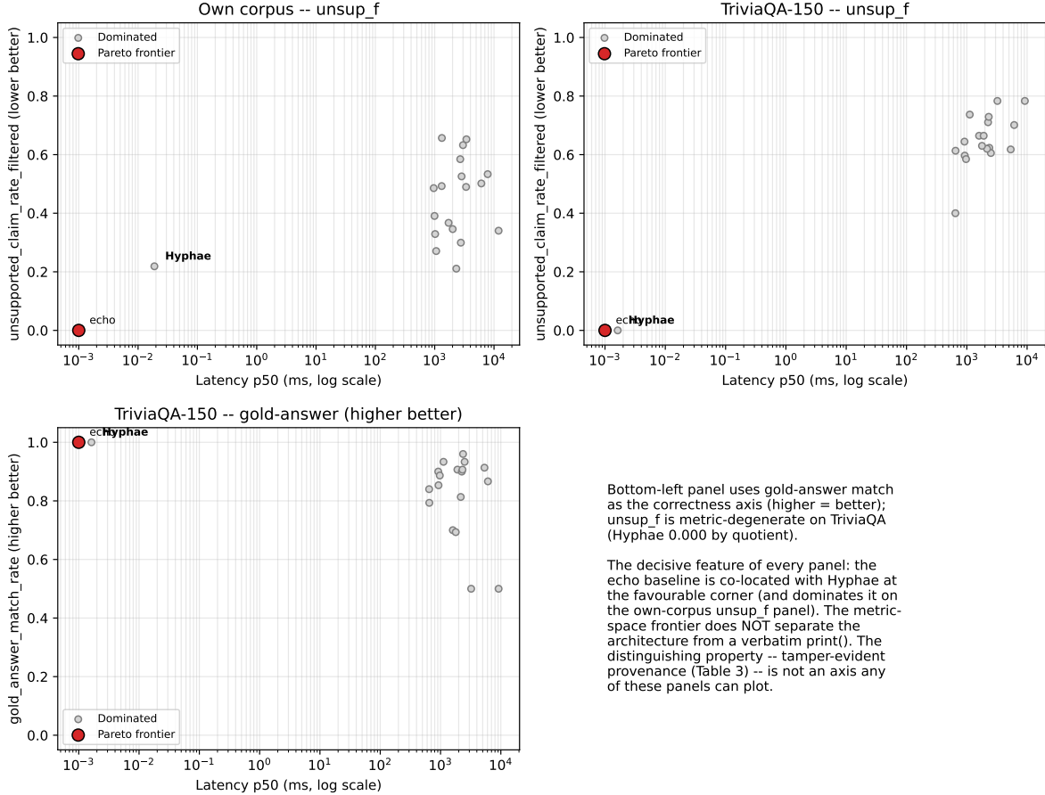
Figure 1: Latency-quality frontier on two metrics, with the echo control. Each point is one system configuration; latency on the horizontal axis is p50 in milliseconds, log scale. Top row uses unsup_f (lower better); bottom-left uses gold-answer match (higher better). Red points are non-dominated. The echo baseline sits at the same favourable corner as HYPHAE (and dominates it on the own-corpus unsup_f panel): the metric-space frontier does not separate the architecture from a verbatim print . The distinguishing property — hash-chained provenance — is not an axis any of these panels can plot.
