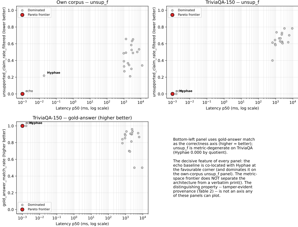
Figure 1: Latency-quality frontier on two metrics, with the echo control. Each point is one system configuration; latency on the horizontal axis is p_{50} in milliseconds, log scale. The top row uses unsup_f and is illustrative only : unsup_f is metric-degenerate for verbatim systems (Hyphae and echo both reach 0.000 on TriviaQA by quotient; §5.1), so the load-bearing correctness axis is the bottom-left panel, gold-answer match (higher better). Red points are non-dominated. On every panel the echo baseline sits at the same favourable corner as HYPHAE (and dominates it on the own-corpus unsup_f panel): the metric-space frontier does not separate the architecture from a verbatim print . The distinguishing property — tamper-evident provenance, measured in Table 2 — is not an axis any of these panels can plot.
