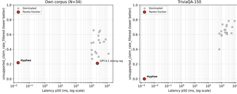
Figure 1: Latency-quality Pareto frontier. Each point is one system configuration. Latency on the horizontal axis is p_{50} in milliseconds, log scale. Vertical axis is unsup_f , lower better. The non-dominated frontier on TriviaQA contains only HYPHAE; on the own corpus it contains HYPHAE and GPT-4.1 with strong retrieval. Other systems are dominated on at least one of the two axes by one of these two points.
