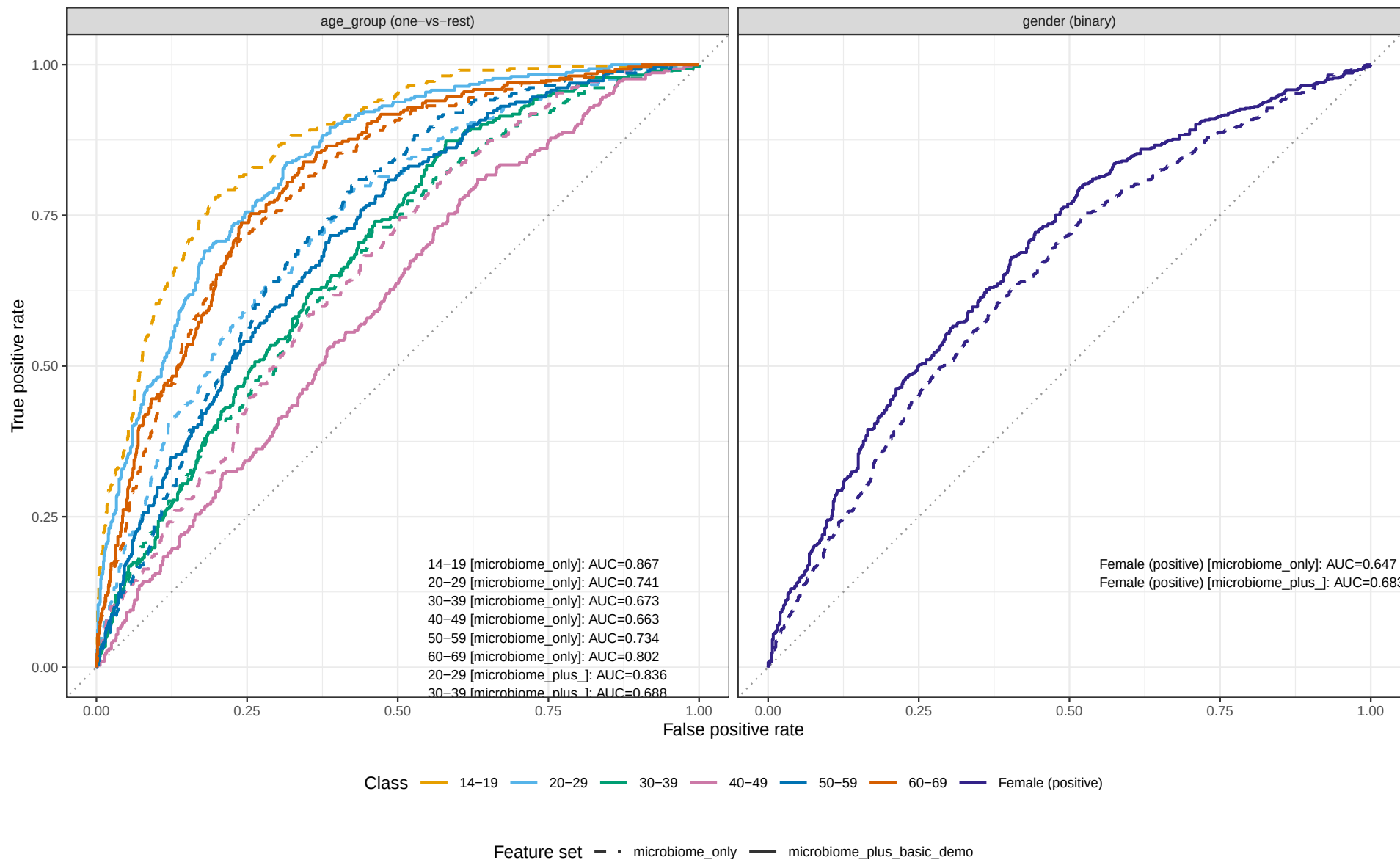
ROC curves -- all classification tasks (test set)
