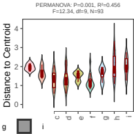
C Centroid Distance
