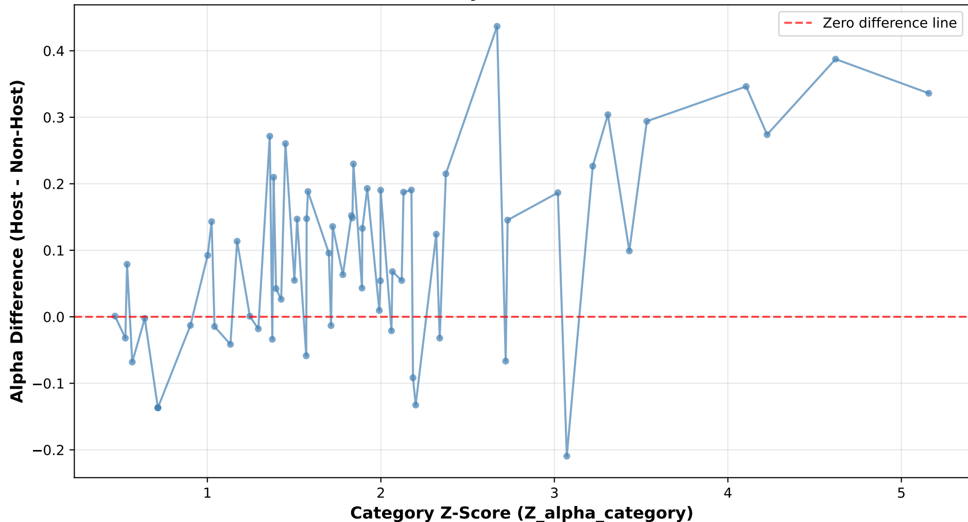
Z-Score vs Host/Non-Host Alpha Difference (Line Plot) (Pathway Data, R^2 \geq 0.05 )
