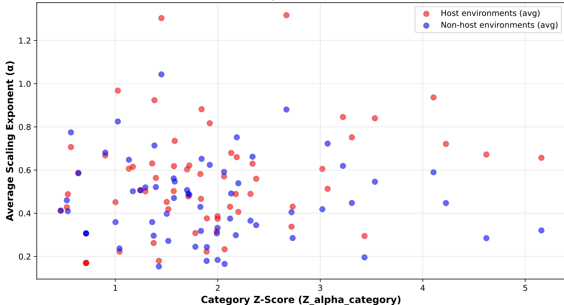
Z-Score vs Average Alpha by Environment Type (Pathway Data, R^2 \geq 0.05 )
