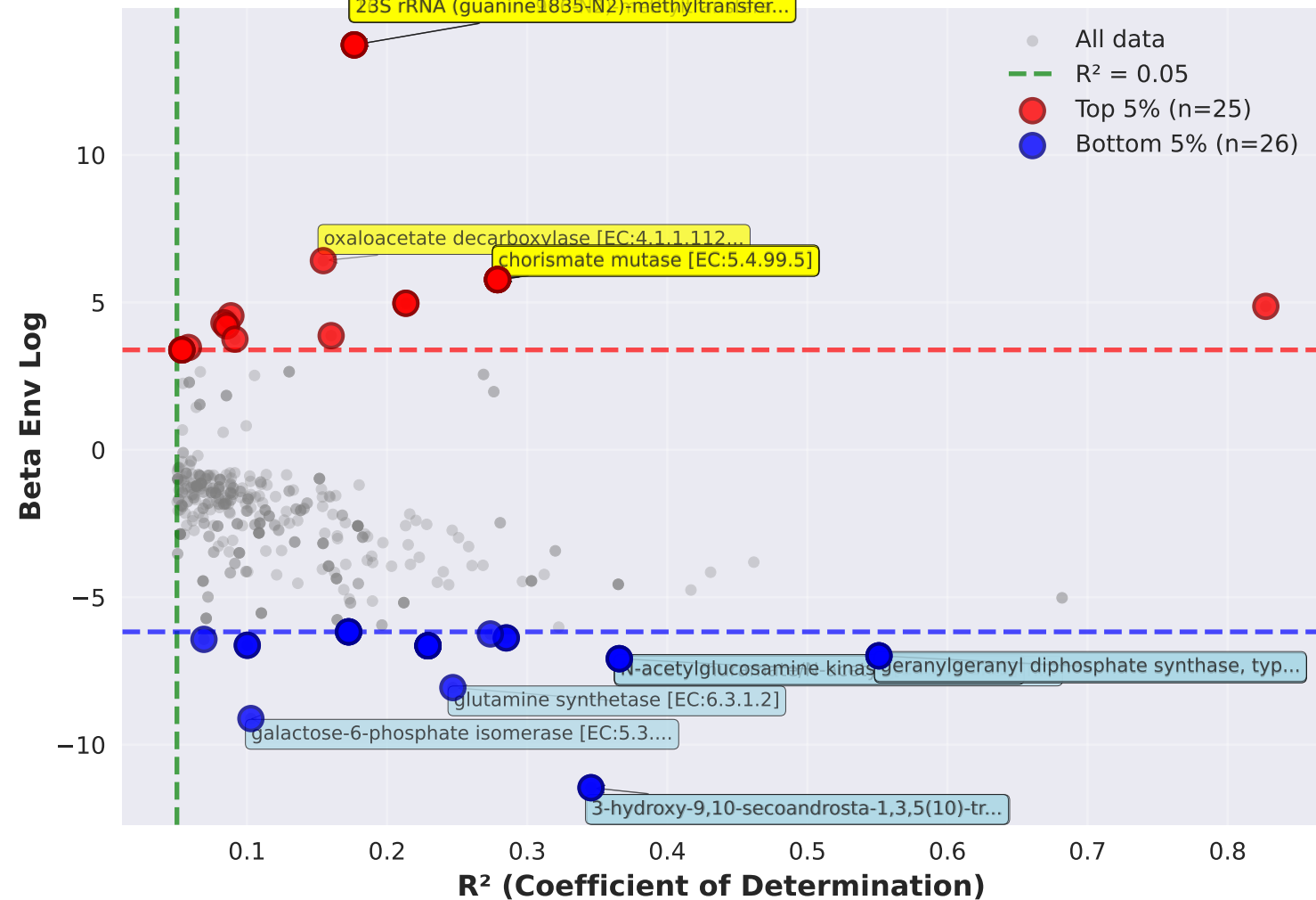
Outlier Categories by Beta Env Log (Host Environments, R^2 \geq 0.05 )
