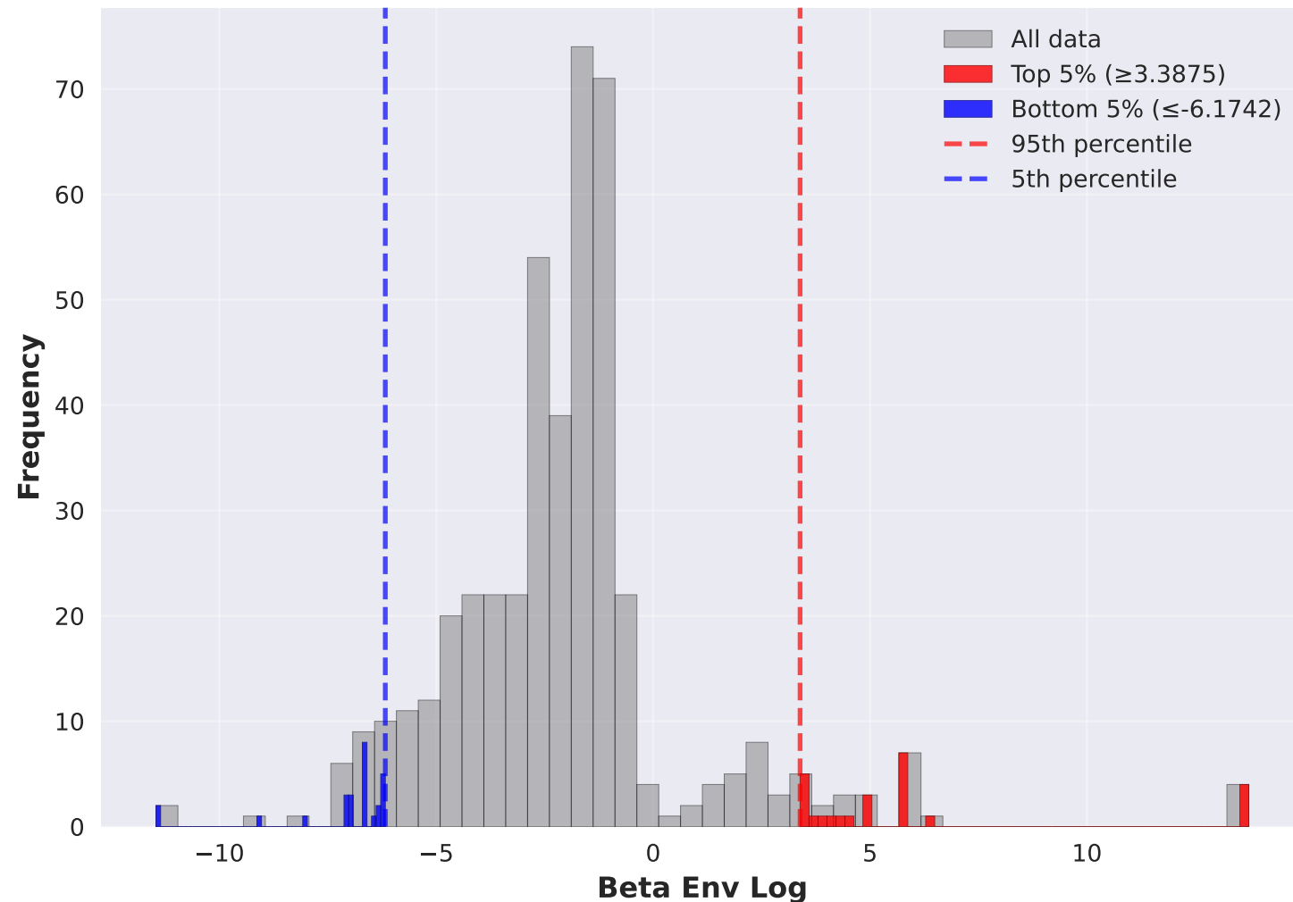
Distribution of Beta Env Log (Host Environments, R^2 \geq 0.05 )
