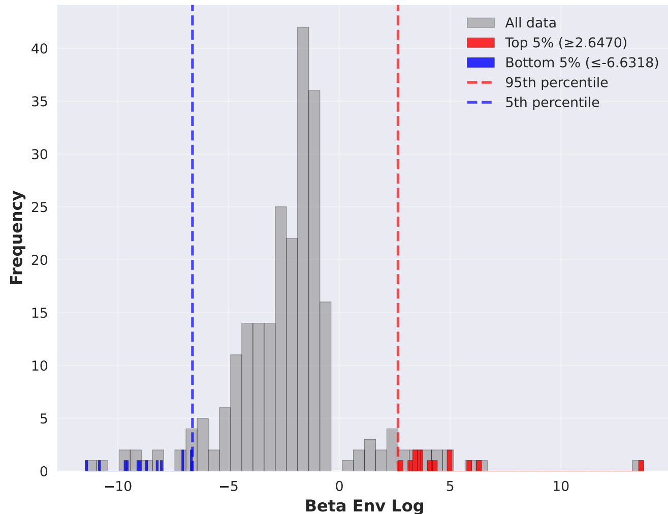
Distribution of Beta Env Log (Host Environments, R^2 \geq 0.05 )
