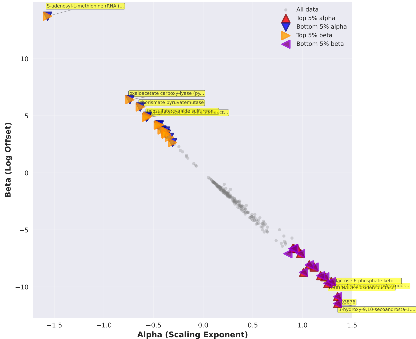
Host Environments (Mammals, Mammals: Human, Plants)
