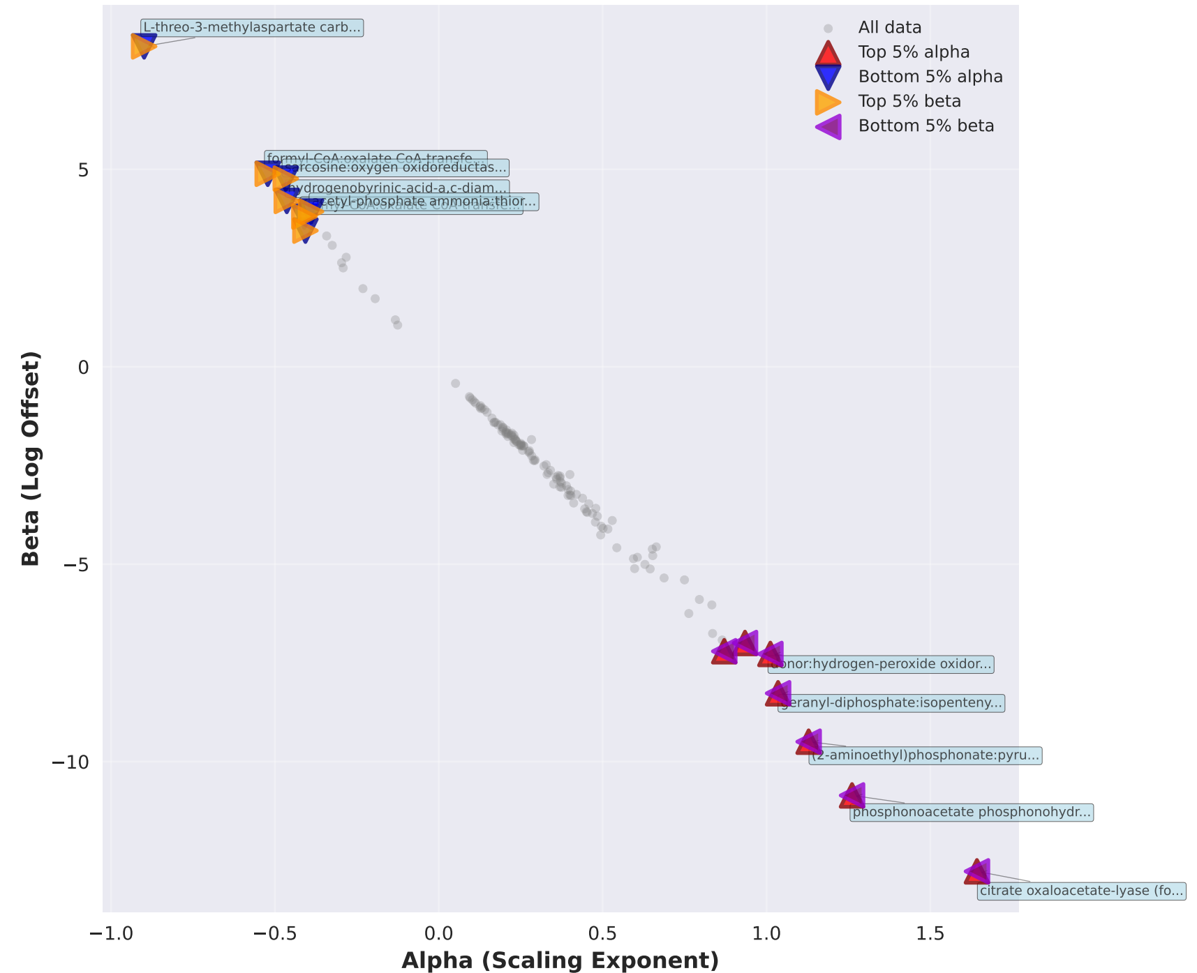
Non-Host Environments (Aquatic, Terrestrial)
