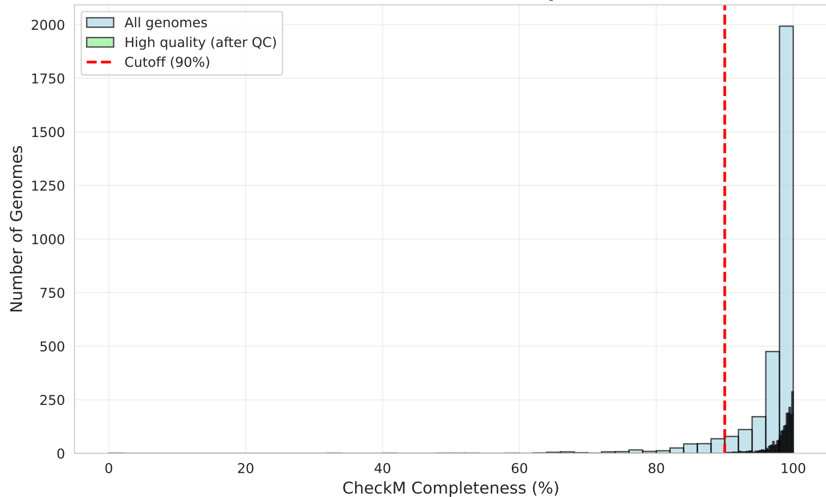
Distribution of CheckM Completeness
