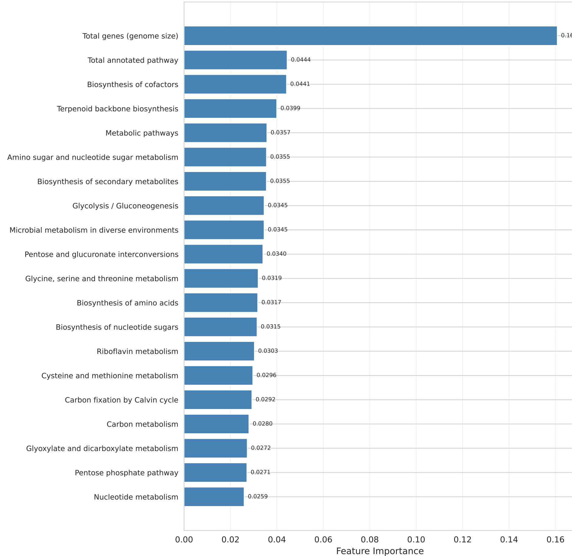
GB Top 20 Features
