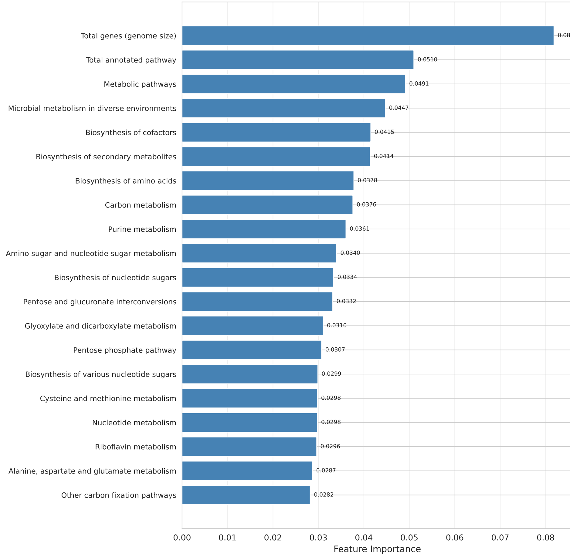
RF Top 20 Features
