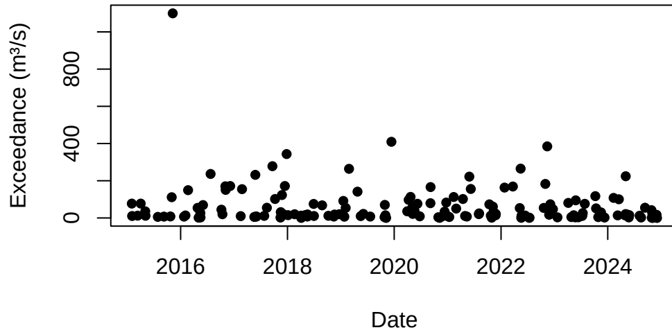
Figure 5: River flow exceedances above 75 cumecs over time.
