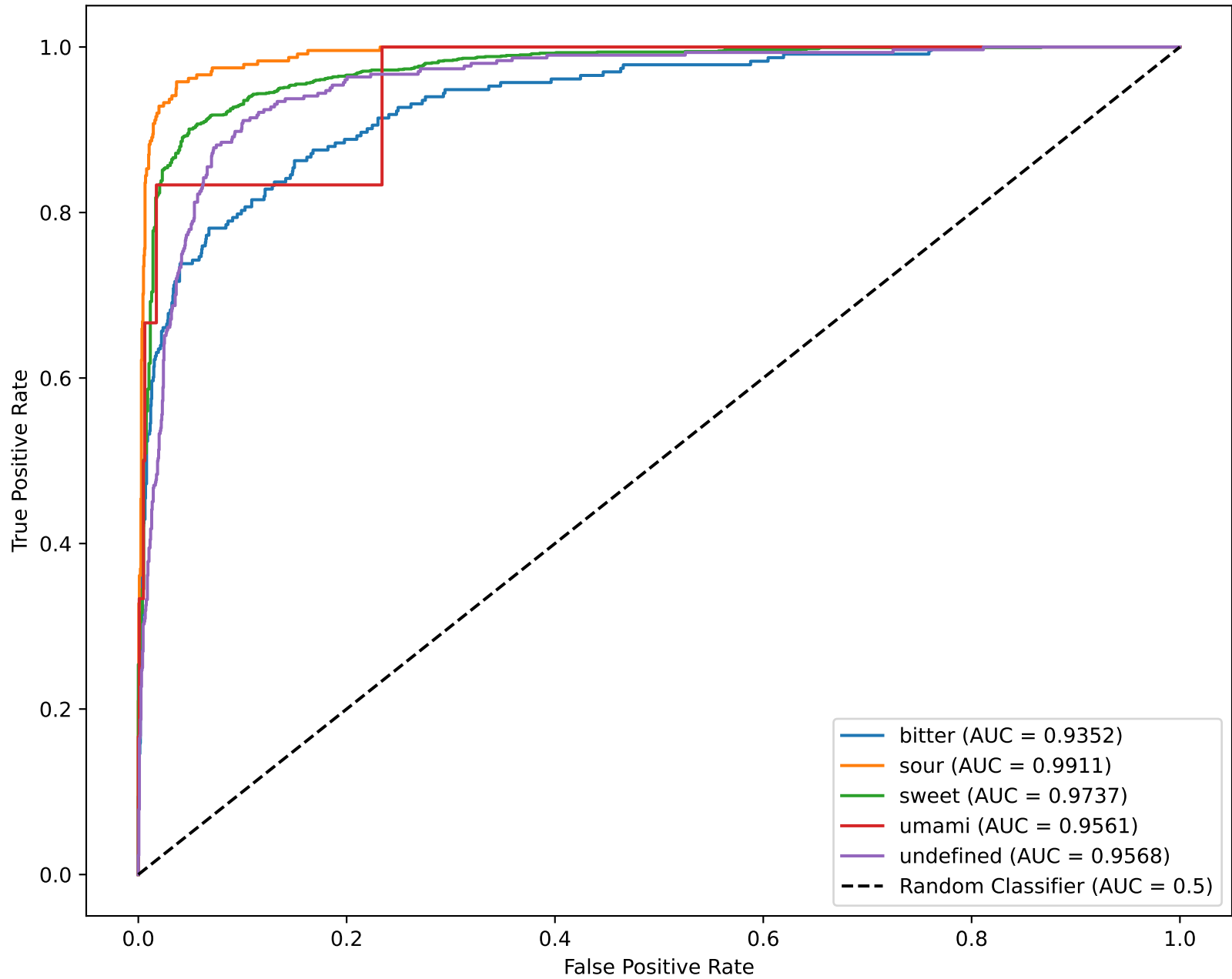
ROC Curves for Each Class
