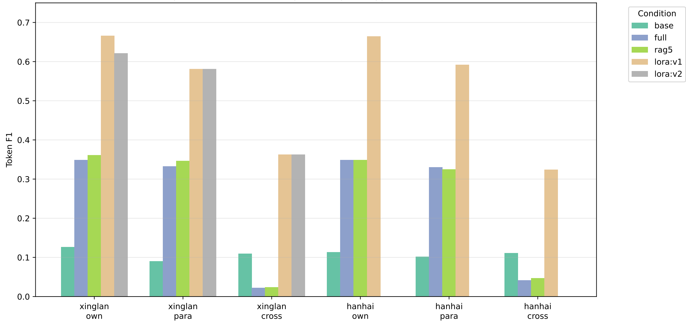
Synthetic Wiki: token F1 by tenant, probe type, and condition
