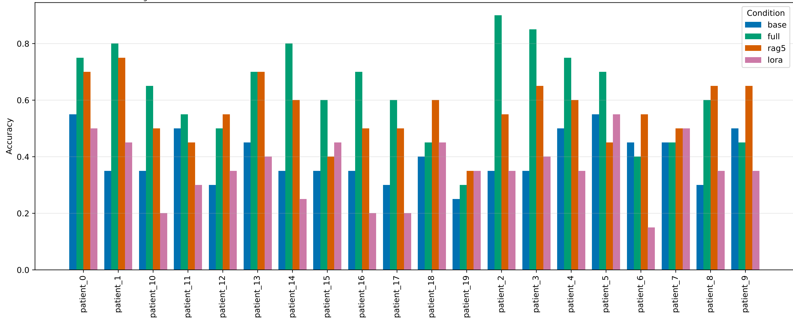
LongHealth: Per-Patient Accuracy (20 patients, 20 questions each)
