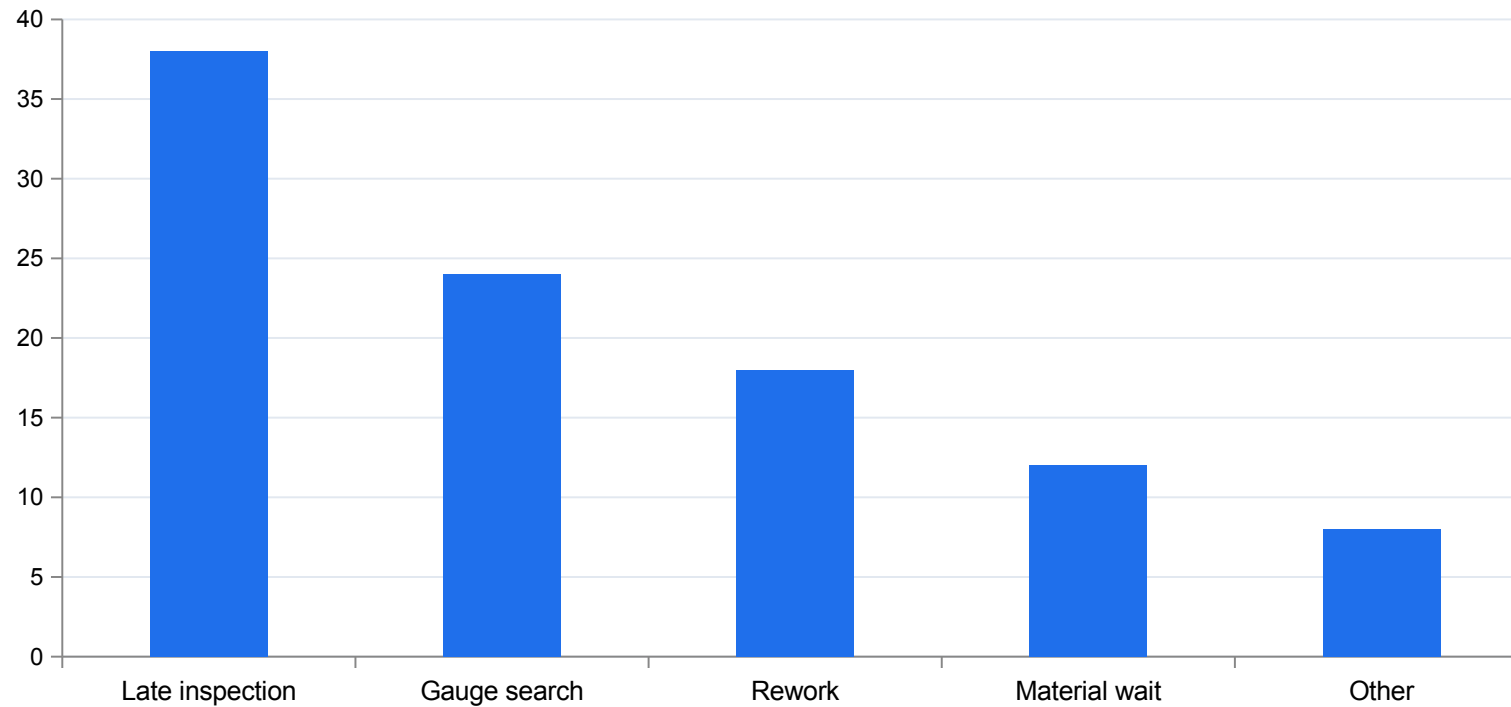
Observed value
