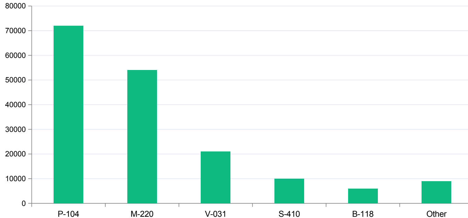
Observed value
