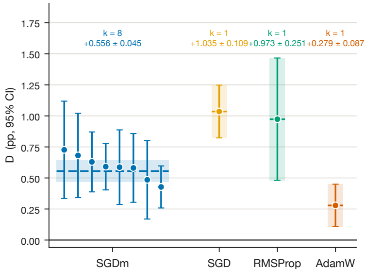
(a) the base optimiser is the moderator
