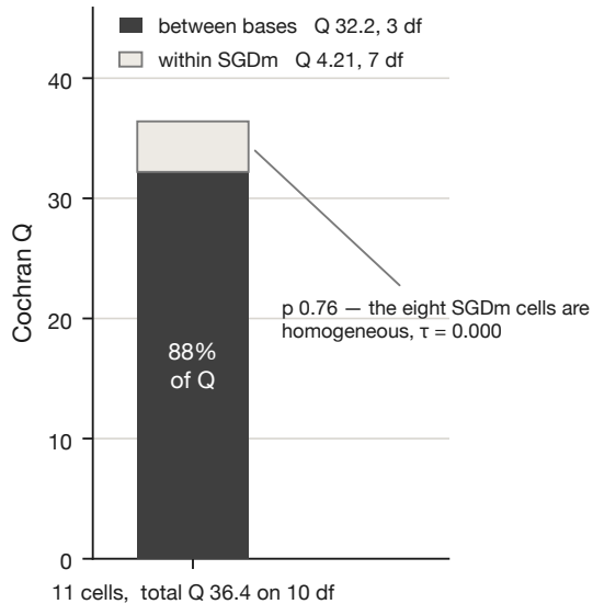
(b) where the heterogeneity lives
