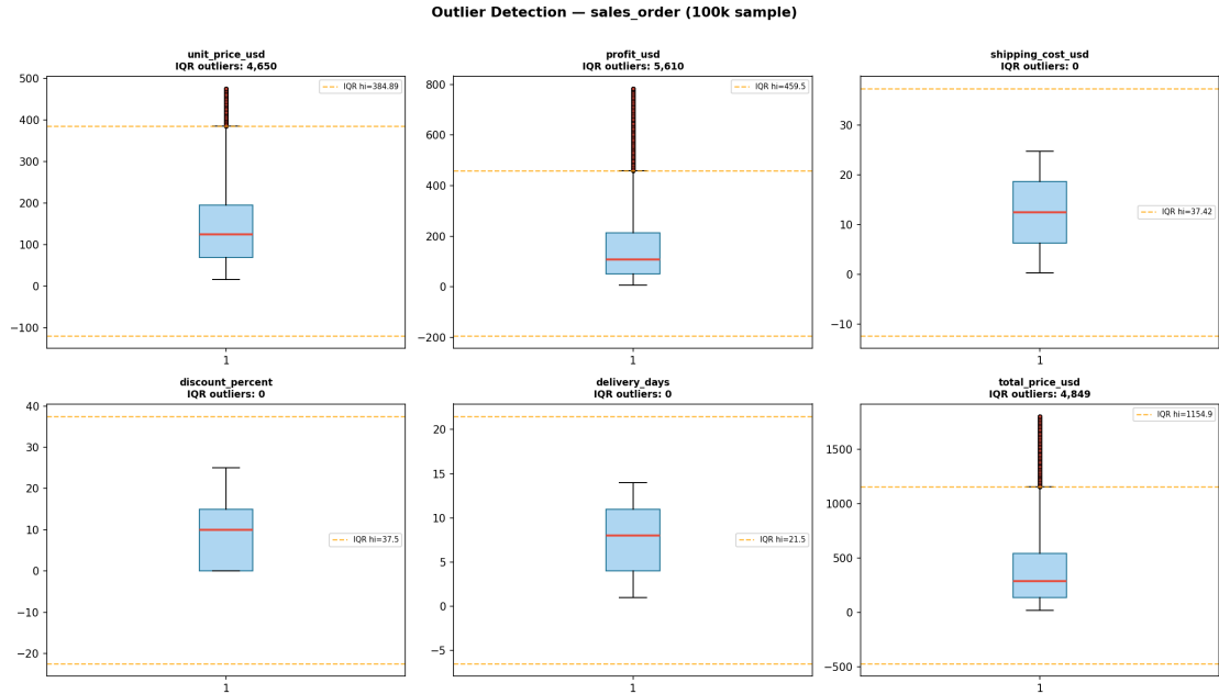
Figure 1.2: DQA outlier detection visualisation
