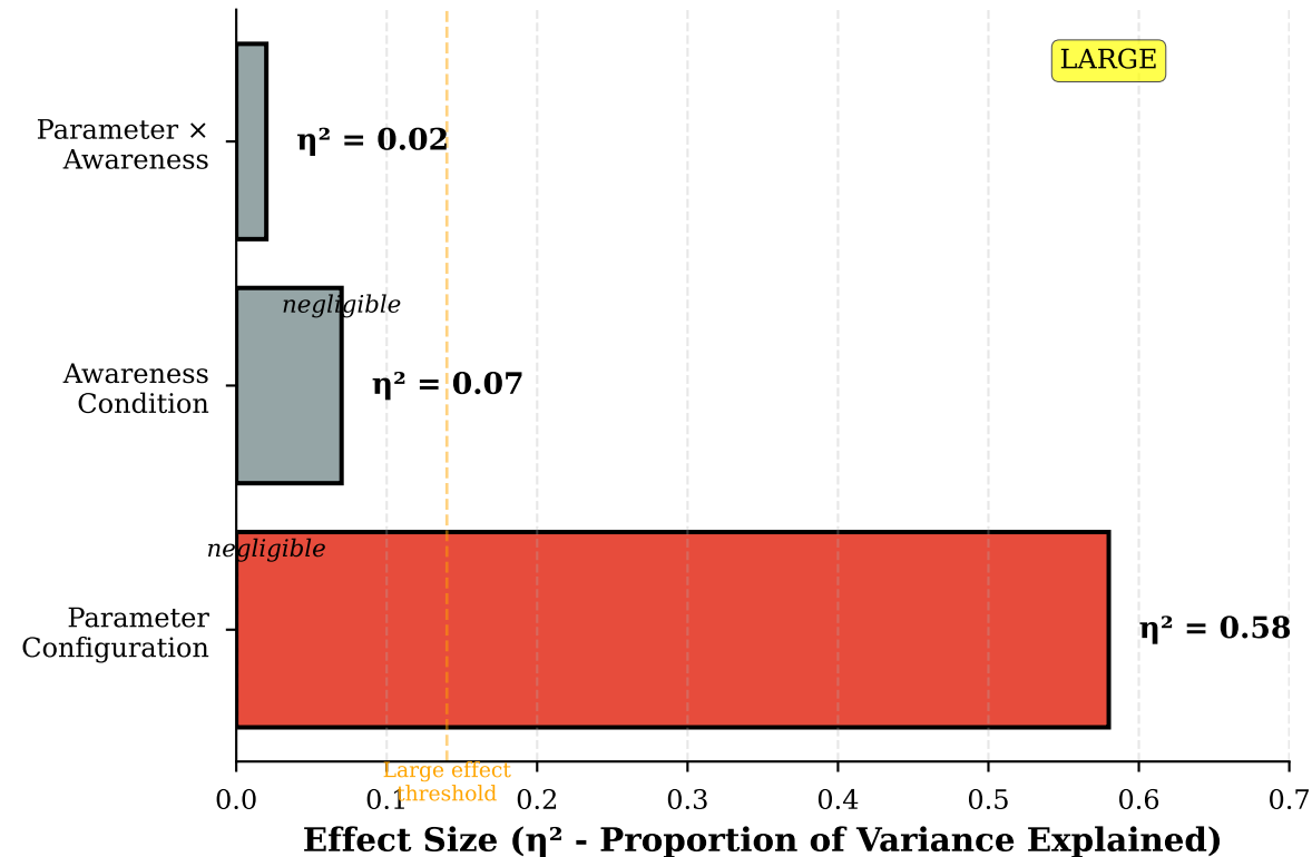
(a) ANOVA Effect Sizes (DV: Authorship Perception)
