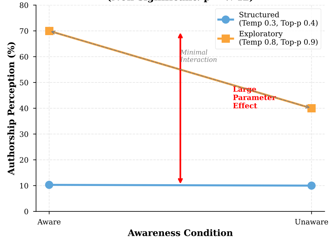
(b) Parameter \times Awareness Interaction (Non-significant: p = .742 )
