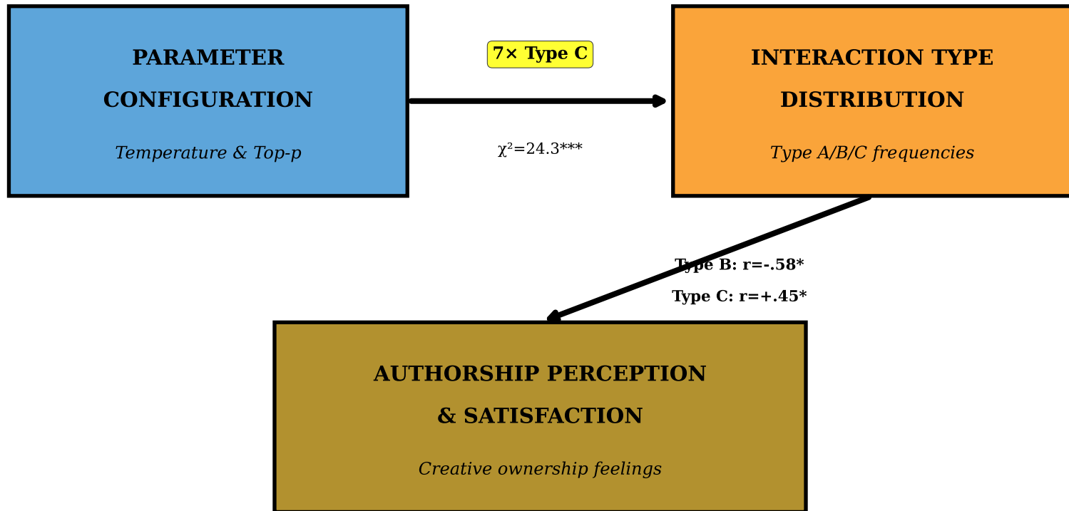
Figure 6: Parameter→Interaction→Perception Pathway
