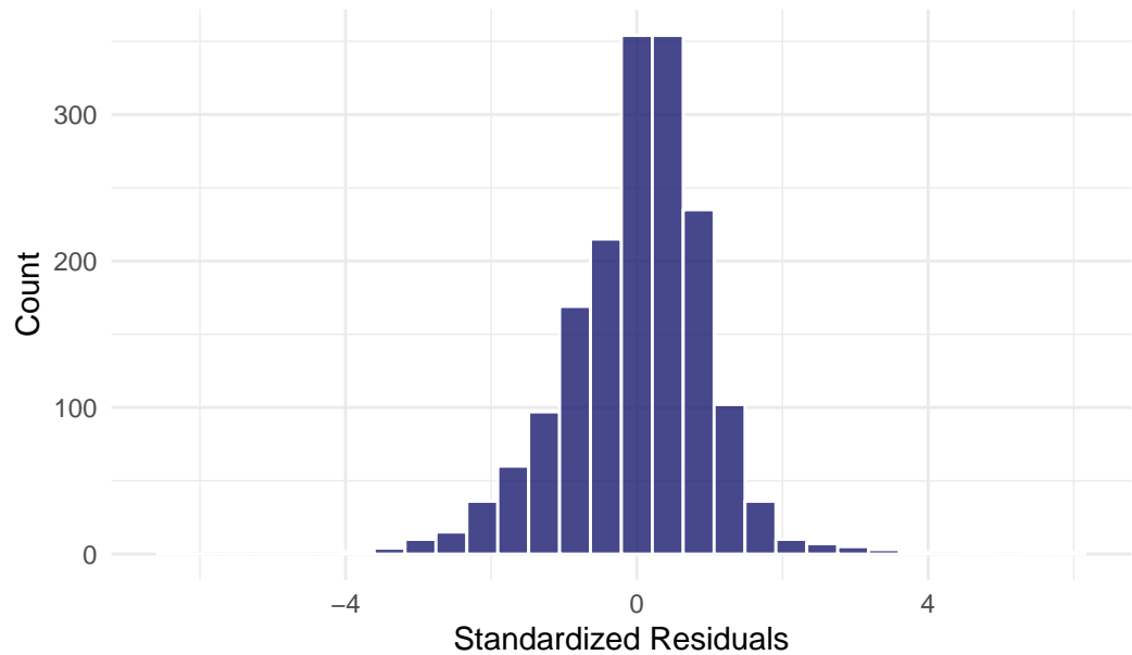
Histogram of Standardized Residuals
