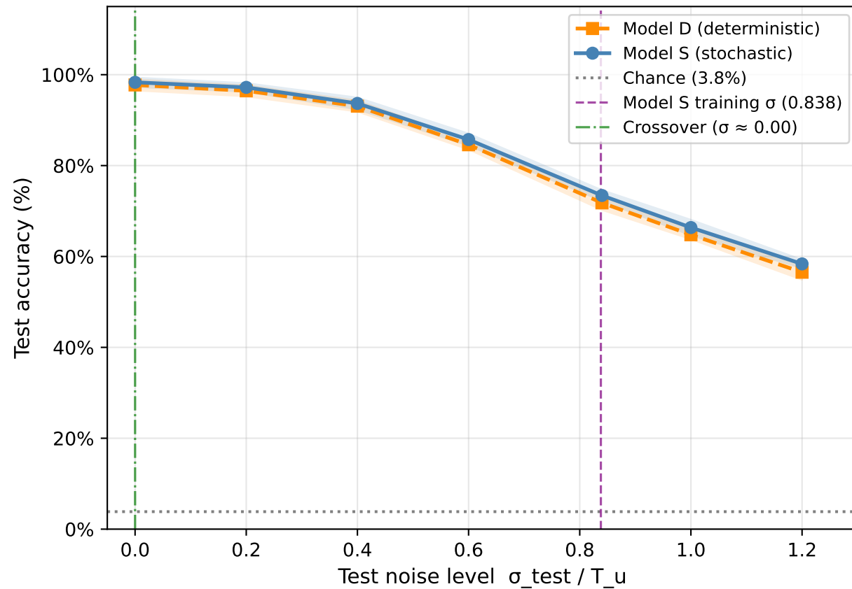
Experiment 3: Stochastic Training — Main Test (stochastic \omega , r ) (mean \pm std, 10 seeds, 500 train / 100 test per class)
