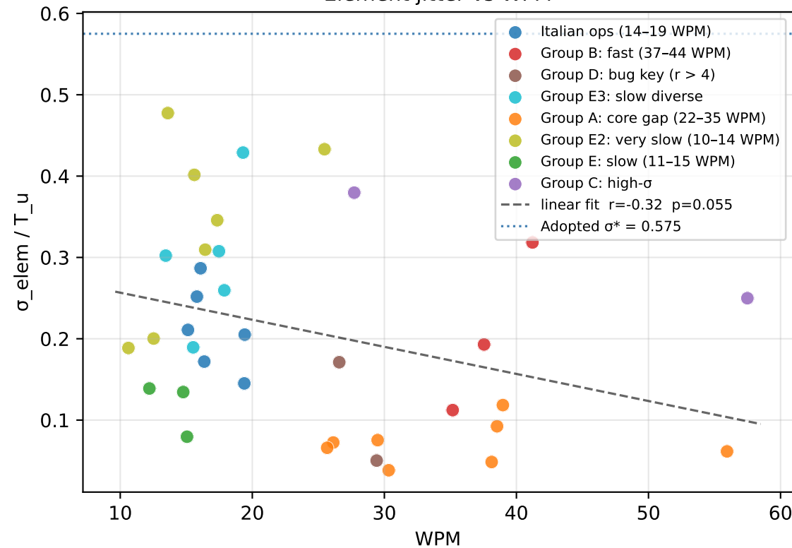
Element jitter vs WPM
