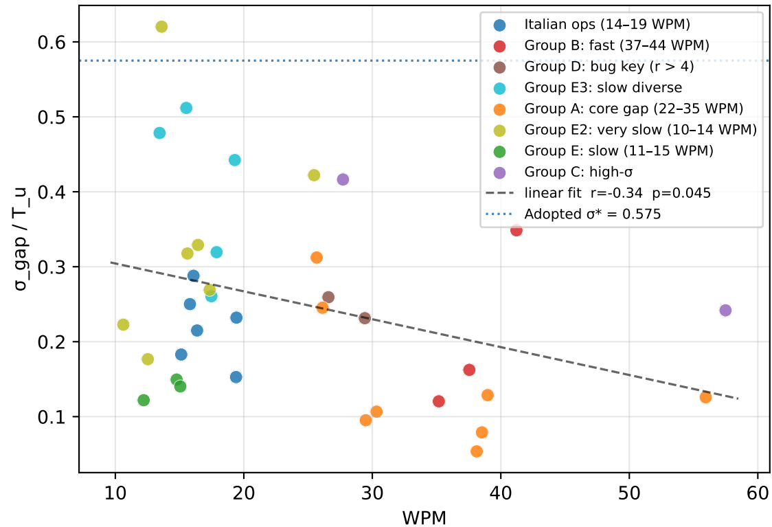
Gap jitter vs WPM
