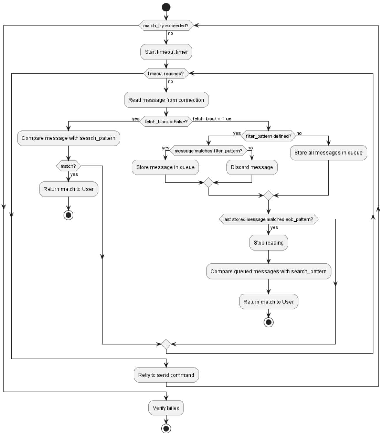
Figure 2.2: Verify workflow
