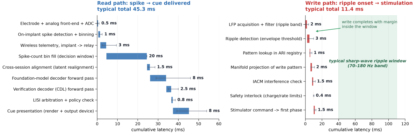
Figure 2: Closed-loop latency budget. Read path (left) and write path (right), stage by stage, with min/max whiskers. The write chain’s worst case (28.0 ms) fits inside a hippocampal ripple event. All values are computed from the formulas in Table 3; none is measured.
