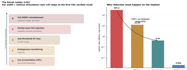
Figure 3: Left: the intervention ladder, bar width proportional to relative stimulation cost; LISI stops at the first CDL-verified recall. Right: why data reduction must happen on the implant — broadband telemetry exceeds any implantable wireless budget by orders of magnitude.
